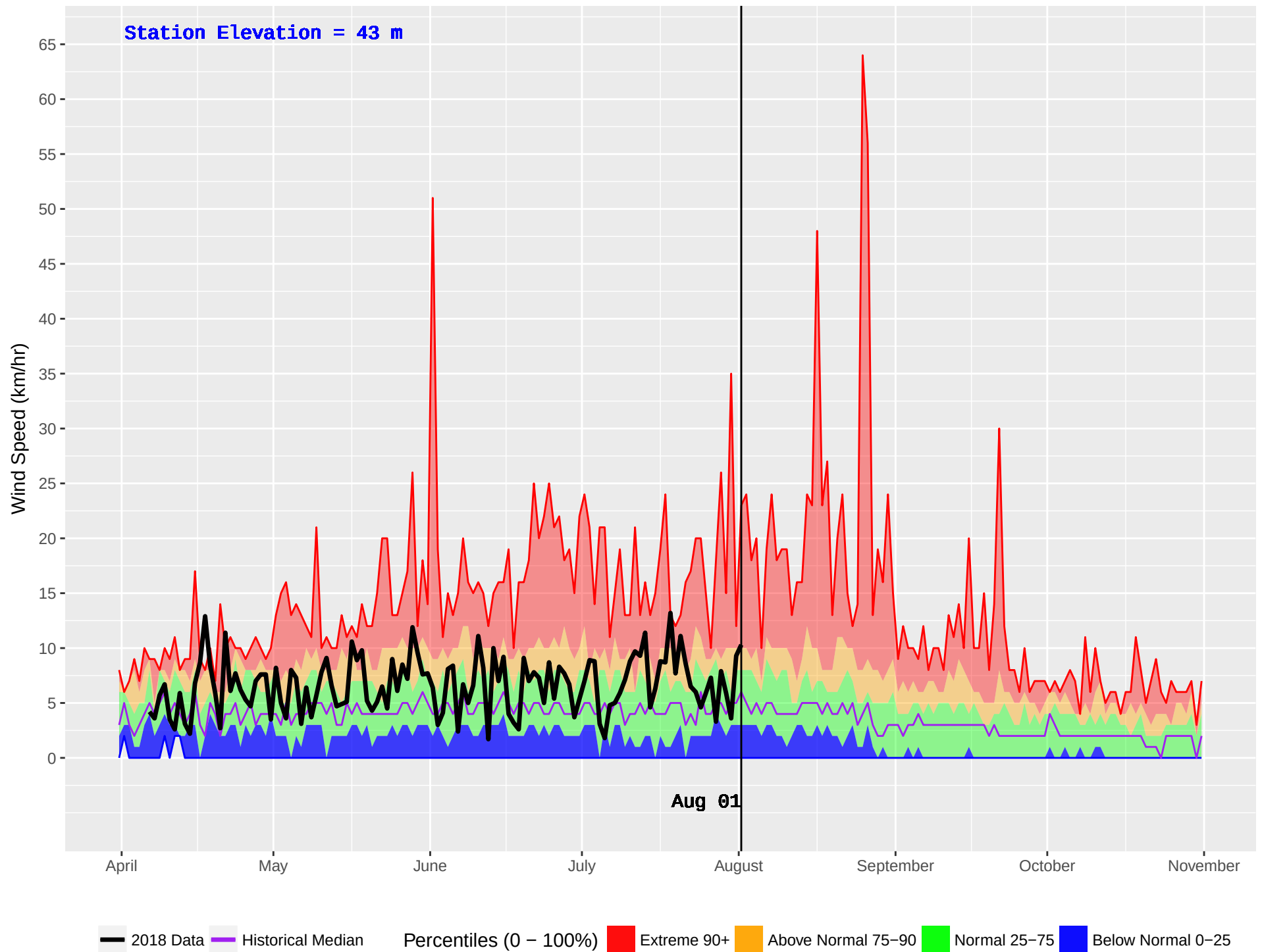
TOBA CAMP (75) : Historical (1970–2016) and Current (2018) Daily Wind Speed
